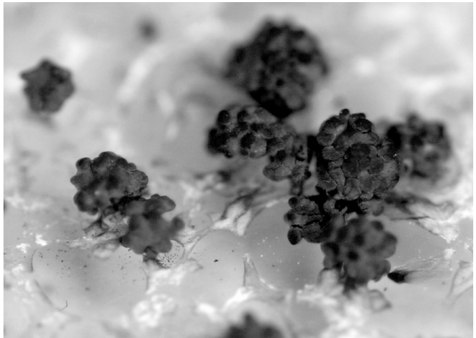
Sporangia of Physarum
